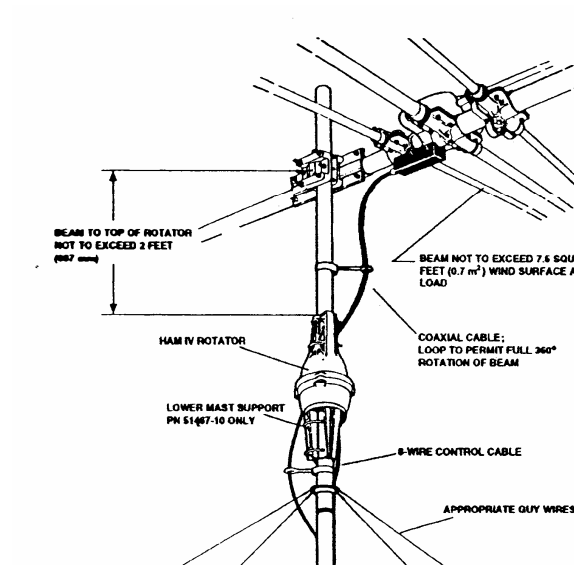
Pole Mounted Rotator
