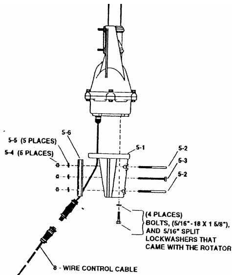
Rotator Mounting with Mast Support With Cable Routing
